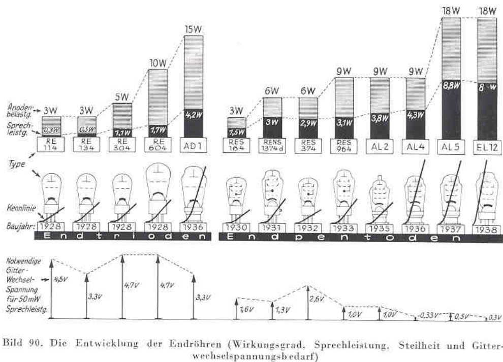
Fig. 11 Comparison of Output tubes (taken from [4] )
