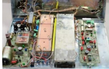
328-Yaesu-SSB Transciver-FT-200
