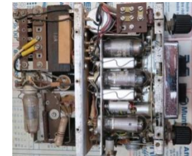
248-Philips-Sport-NDK372V
