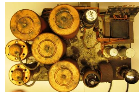
180-Philips-Super Inductance-634A
