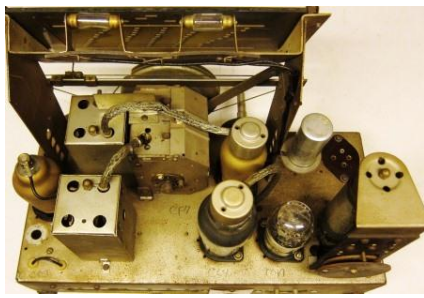
122-Tor-Standard-U48
