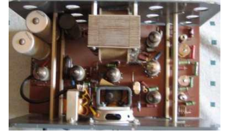
725-KMF-Krystal kalibrator PX781 1960
