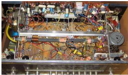
82-B&O-Beomaster 900 K
