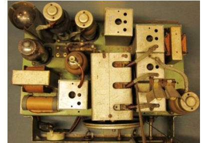
4-Tor-Ultra super-U56
