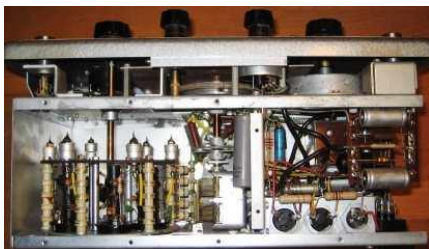
724 Philips HF Oscillator GM2893 1955
