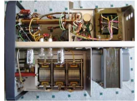
737-Elomar-Signalgenerator-MV604 1940
